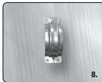
Tailpipe Clamp without Pin Cessna 150 and A150 Replaces: 0450338-10 PN: A0450338-10 PMA New-outright: $11 Can be used for both left and right sides.
